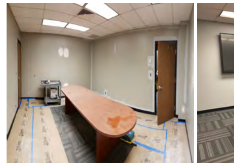
On-Call Architecture
